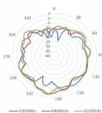
4200-5150 MHz
