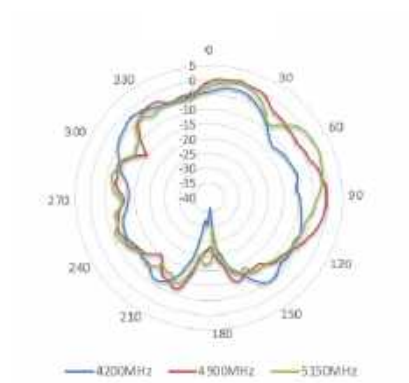
4200-5150 MHz
