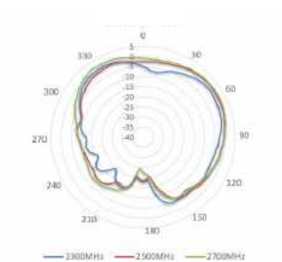
2300-2700 MHz
